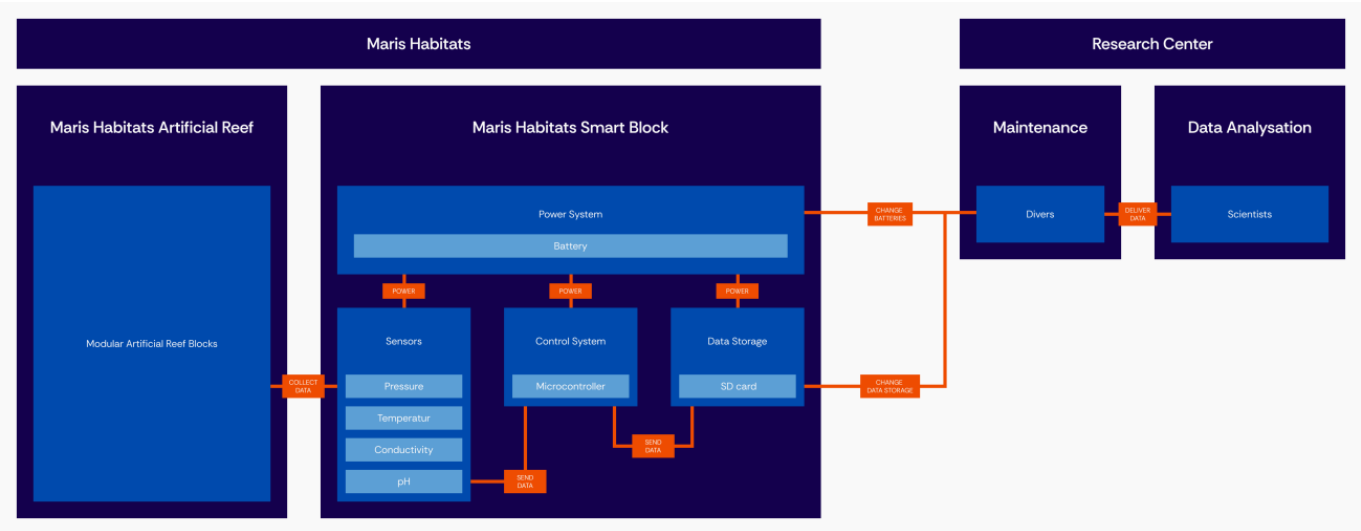
Figure 63: Black Box Diagram V2
