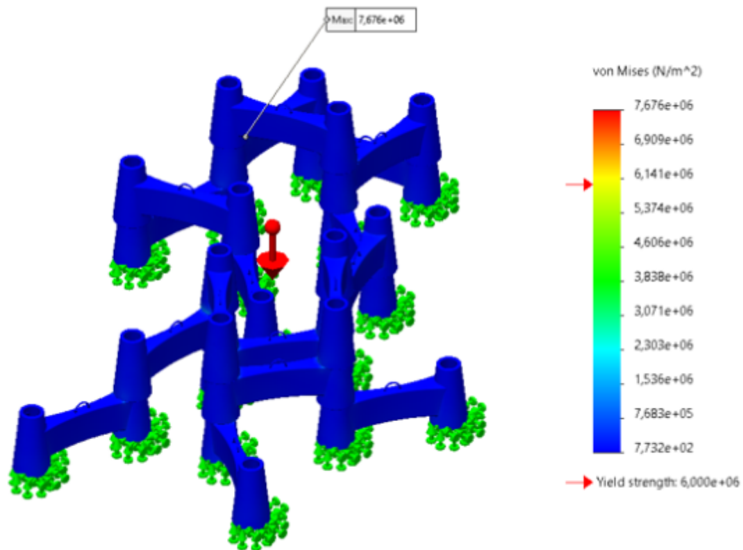
Figure 55: Simulation full structure strength test.
